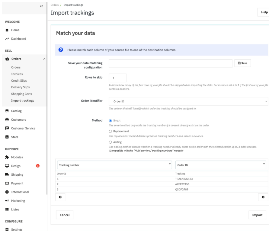
Figure 2: Data matching
